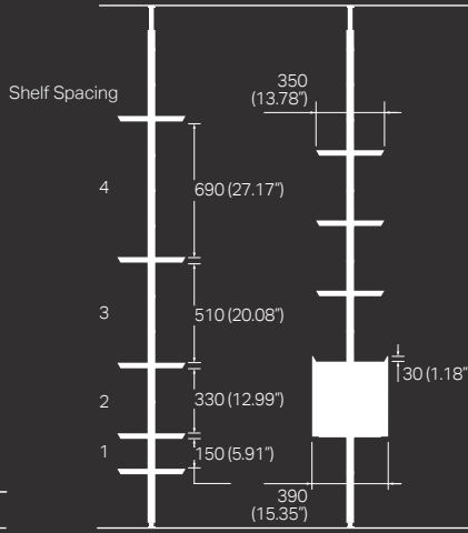
Side view Compression Mounted
