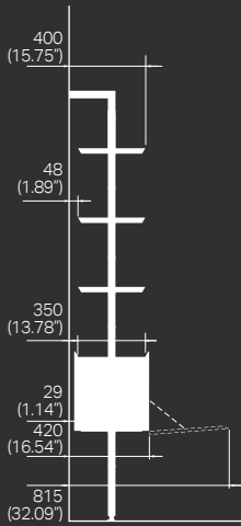
Side view Wall Mounted
